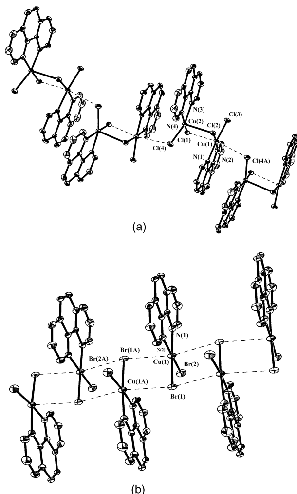
Fig. 3 The one-dimensional chain structures of [CuCl 2 (phen)] 6 and [CuBr 2 (phen)] 8 (30%).
