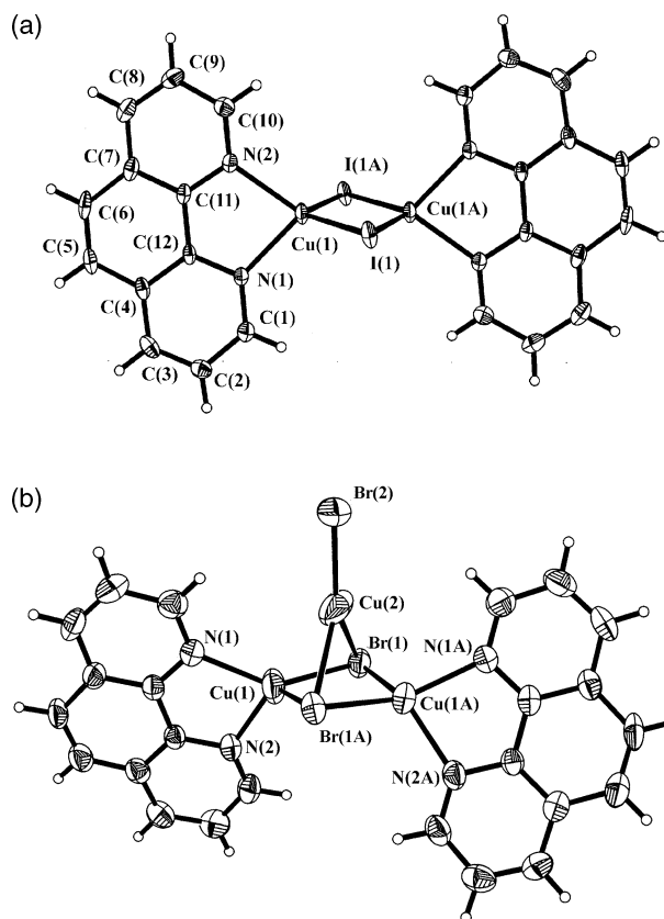
Fig. 2 The molecular structures of dimeric [Cu 2 I 2 (phen) 2 ] 3 and trinuclear [Cu 3 Br 3 (phen) 2 ] 5 (30% probability ellipsoids).
