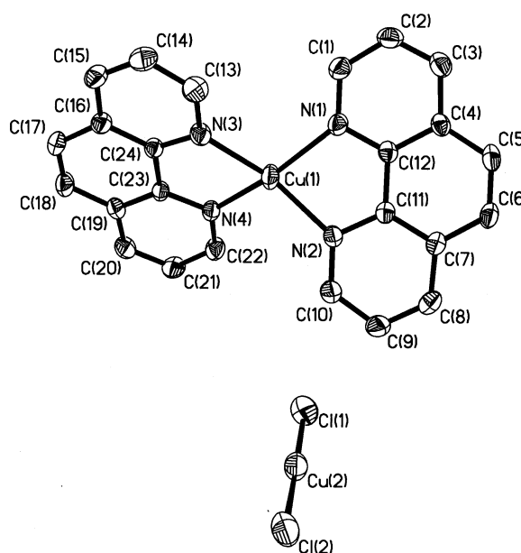
Fig. 1 The molecular structure of ionic [\text{Cu(phen)}_2][\text{CuCl}_2] 1 (30% probability ellipsoids).
