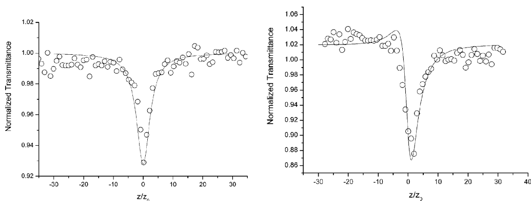
Fig. 4 Z-scan data of 8.85 \times 10^{-4} mol dm -3 of [Cu 3 Br 3 (phen) 2 ] 5 in DMF: (left) collected under the open aperture configuration showing NLO absorption (the solid curve is a theoretical fit); (right) obtained under the closed aperture configuration.
